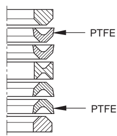
Packing set lower (PTFE) 6004 0266 75
