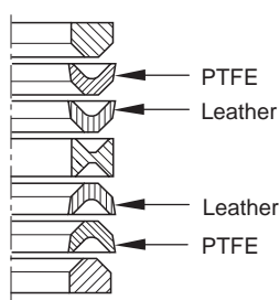
Packing set lower (PTFE + Leather) 6004 0266 77
