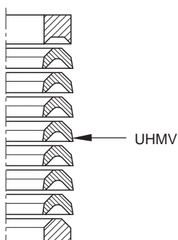
Packing set upper (UHMV) 6004 0266 71
