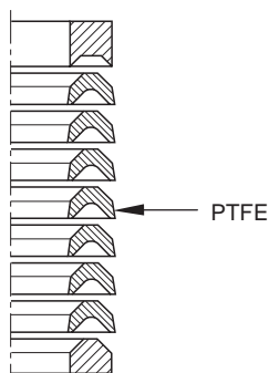
Packing set upper (PTFE) 6004 0266 70
