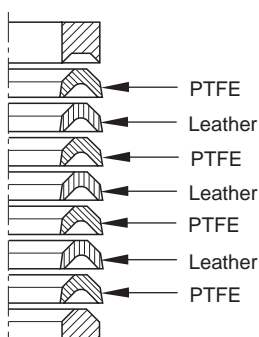
Packing set upper (PTFE + Leather) 6004 0266 72
