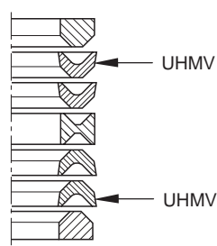
Packing set lower (UHMV) 6004 0266 76
